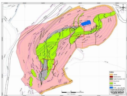
Figure K17: Fibolele Bulk Sampling Pit, surface and geology plan on 31 December 2023
