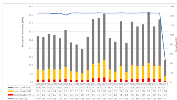
Figure K23: Kagem projected plant feed and recovered gemstones for LoM
