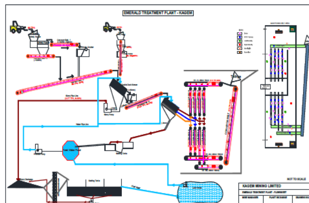
Figure K22: Kagem washing plant schematic flowsheet.
